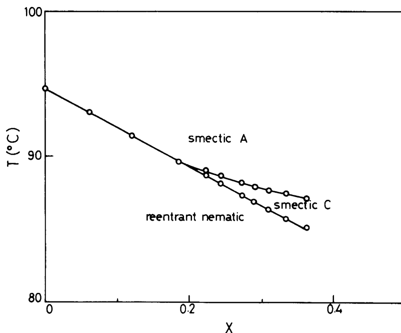
FIGURE 3 Binary phase diagram (at atmospheric pressure) of the liquid crystal mixtures of DOBBCA and 4-cyanobenzylidene-4'-(4''-decyloxybenzoyloxy) aniline. X denotes the mole fraction of DOBBCA in the mixture. (From Sigaud et al. 15 ).
